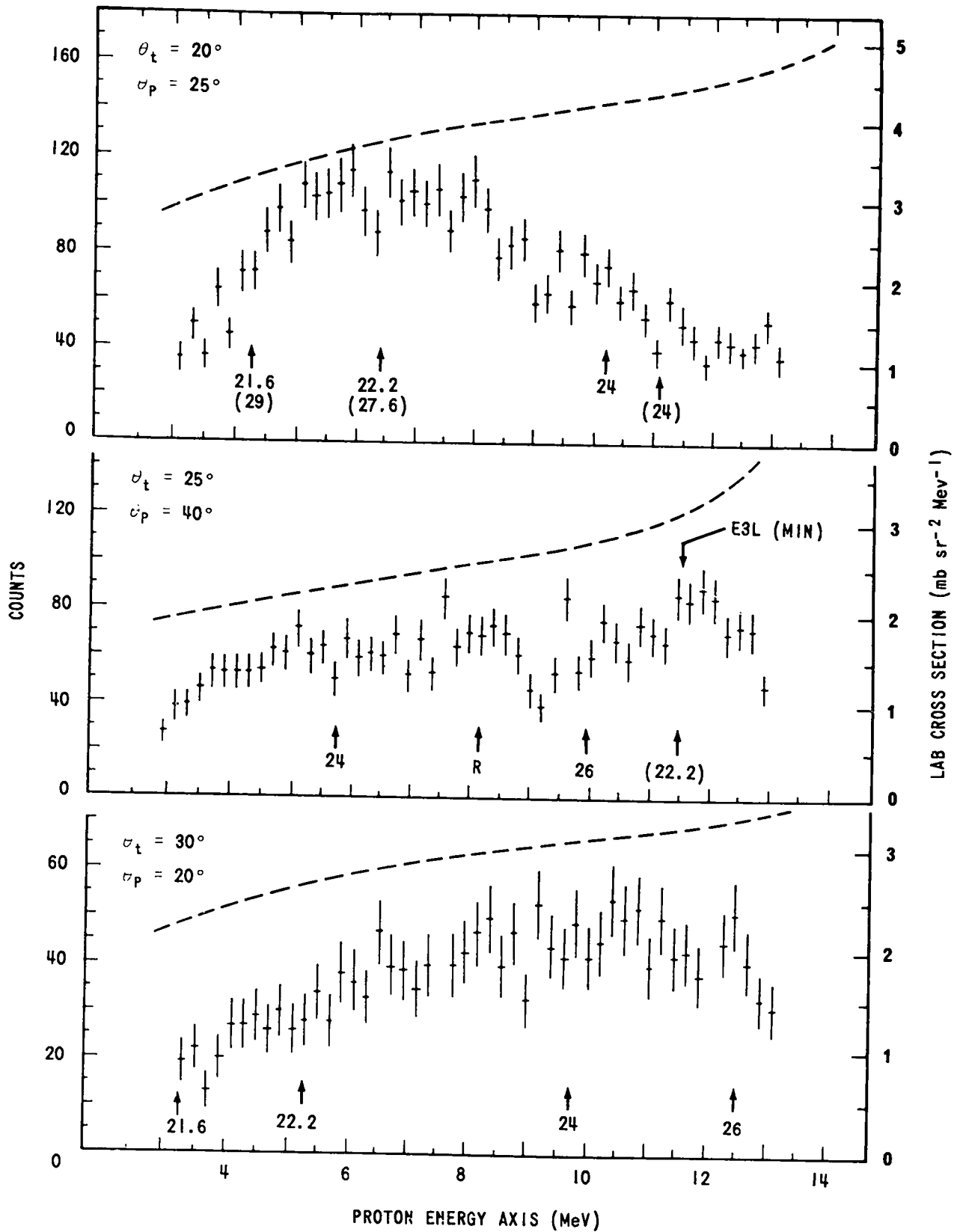
Fig. 9. Projection along the proton axis of additional data from the reaction {}^3\text{He}(d, tp){}^1\text{H} with 20-MeV incident deuterons.
