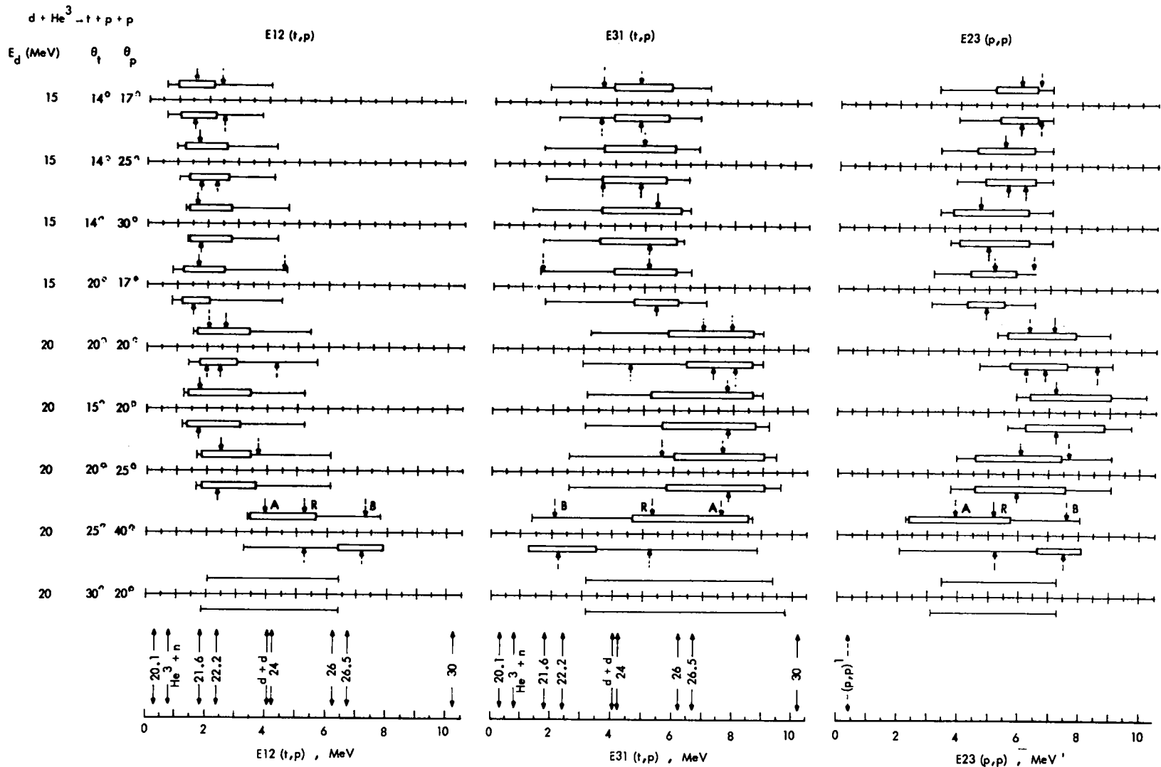
Fig. 19. Graphical summary of the center-of-mass excitation energy information obtained from the ^3\text{He}(d,tp)^4\text{He} data.
