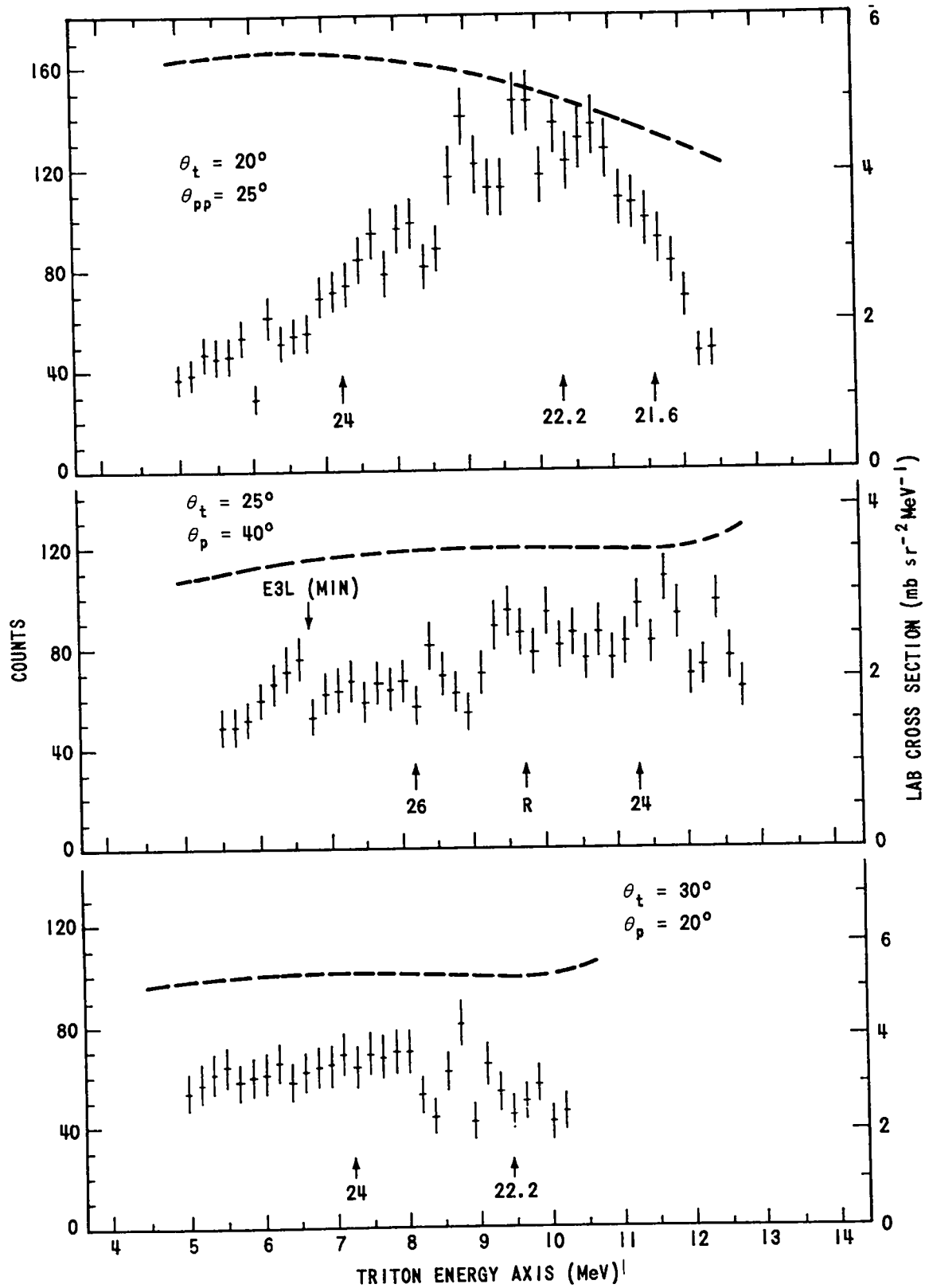
Fig. 8. Projection along the triton axis of additional data from the reaction {}^3\text{He}(d, tp){}^1\text{H} with 20-MeV incident deuterons.
